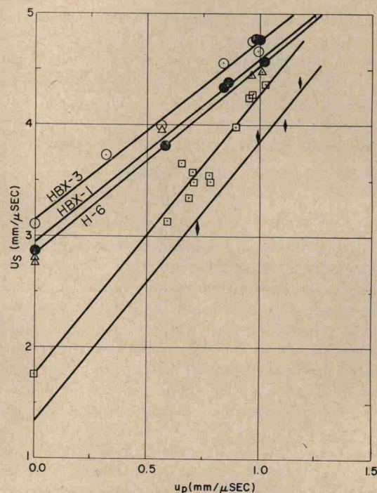
FIG. 9. Shock-wave velocity, U_s , vs particle velocity, u_p , of several aluminized explosives and propellants. O HBX-3, ● HBX-1, △ H-6, □ EJC, ◆ FFP.
