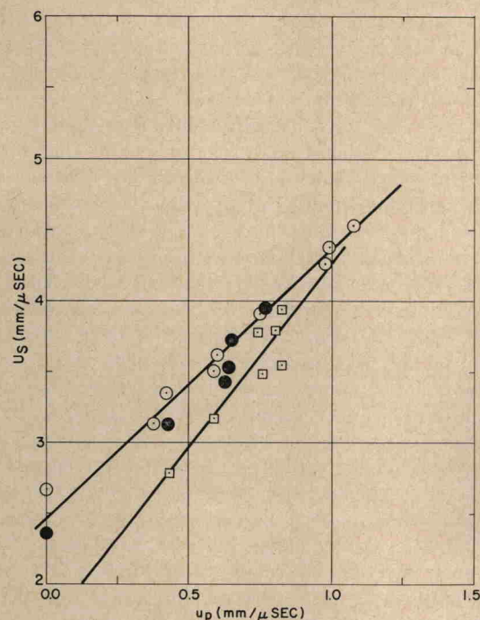
FIG. 8. Shock-wave velocity, U_s , vs particle velocity, u_p , of DATB (O), TNB (●), and TNA/Zytel (□).
